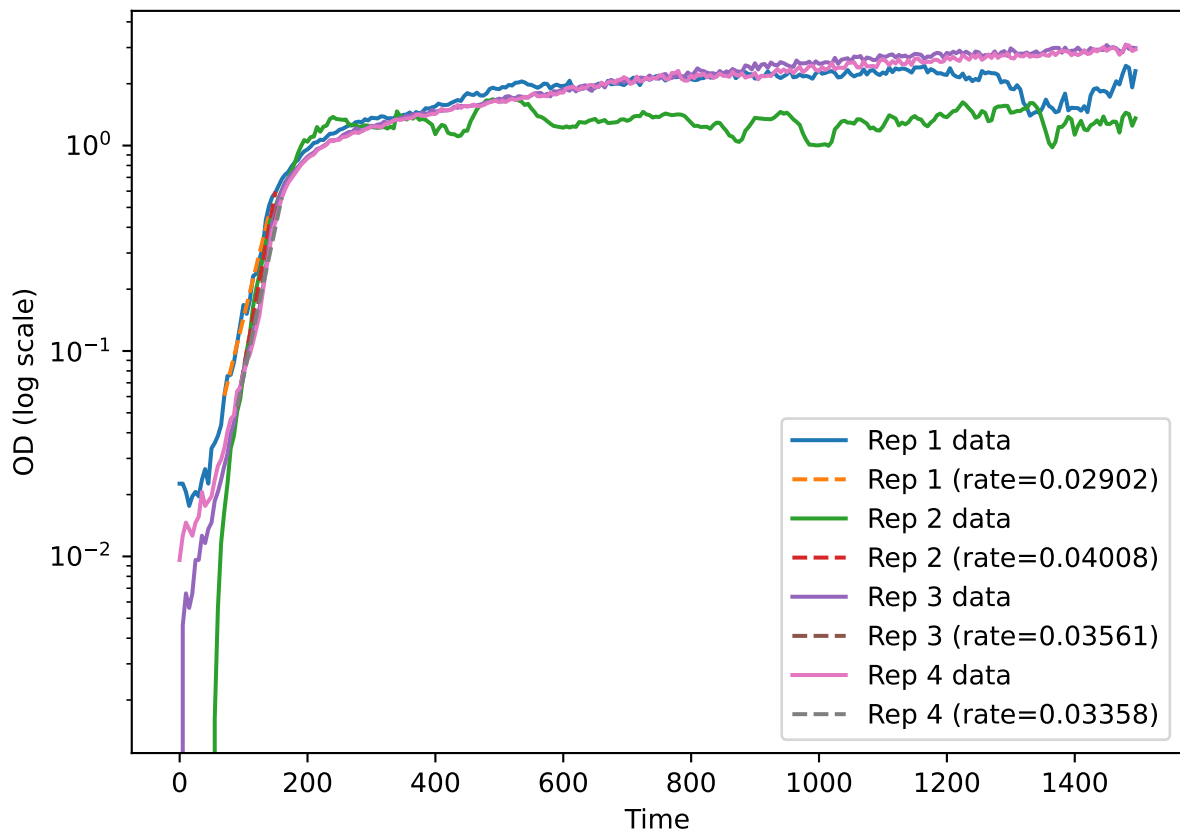
TB194 Cm=2 Growth Curves and Fits
