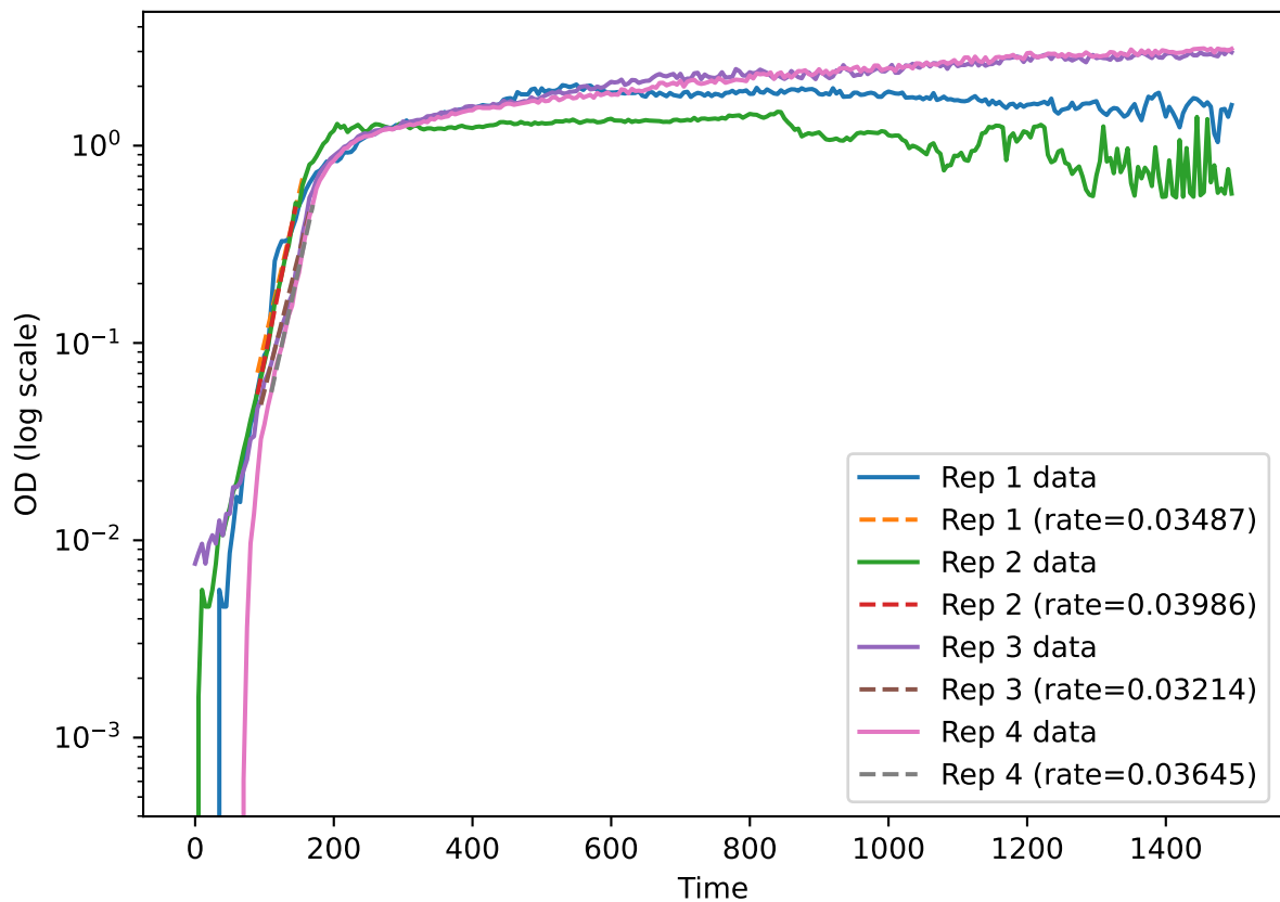
TB194 Cm=4 Growth Curves and Fits
