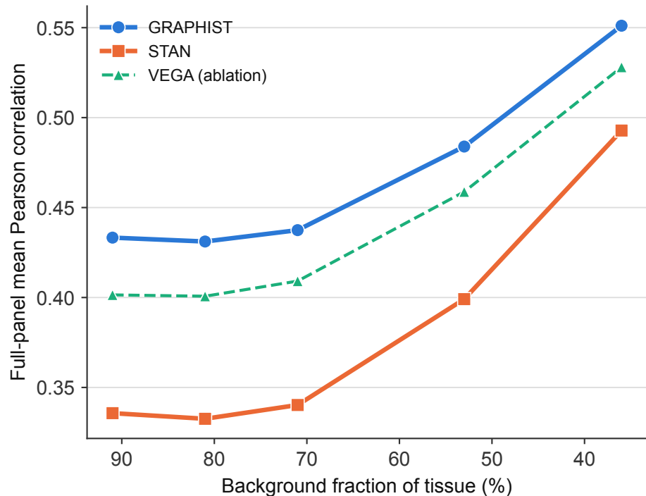
A Absolute recovery accuracy
