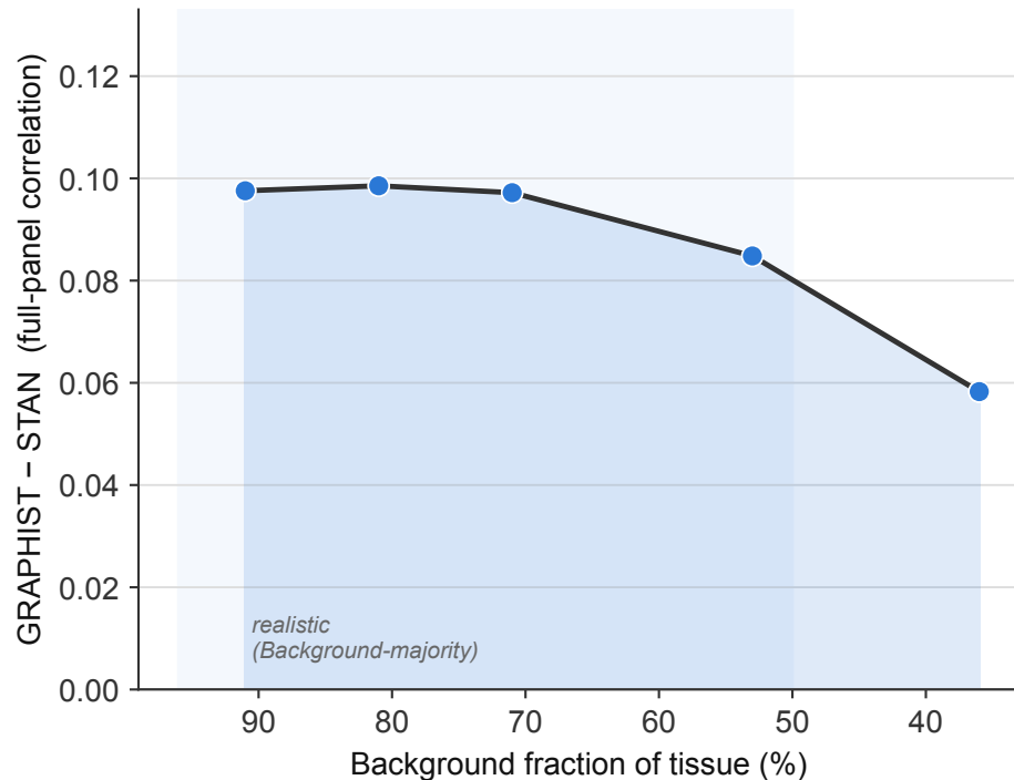
B GRAPHIST's advantage over STAN
