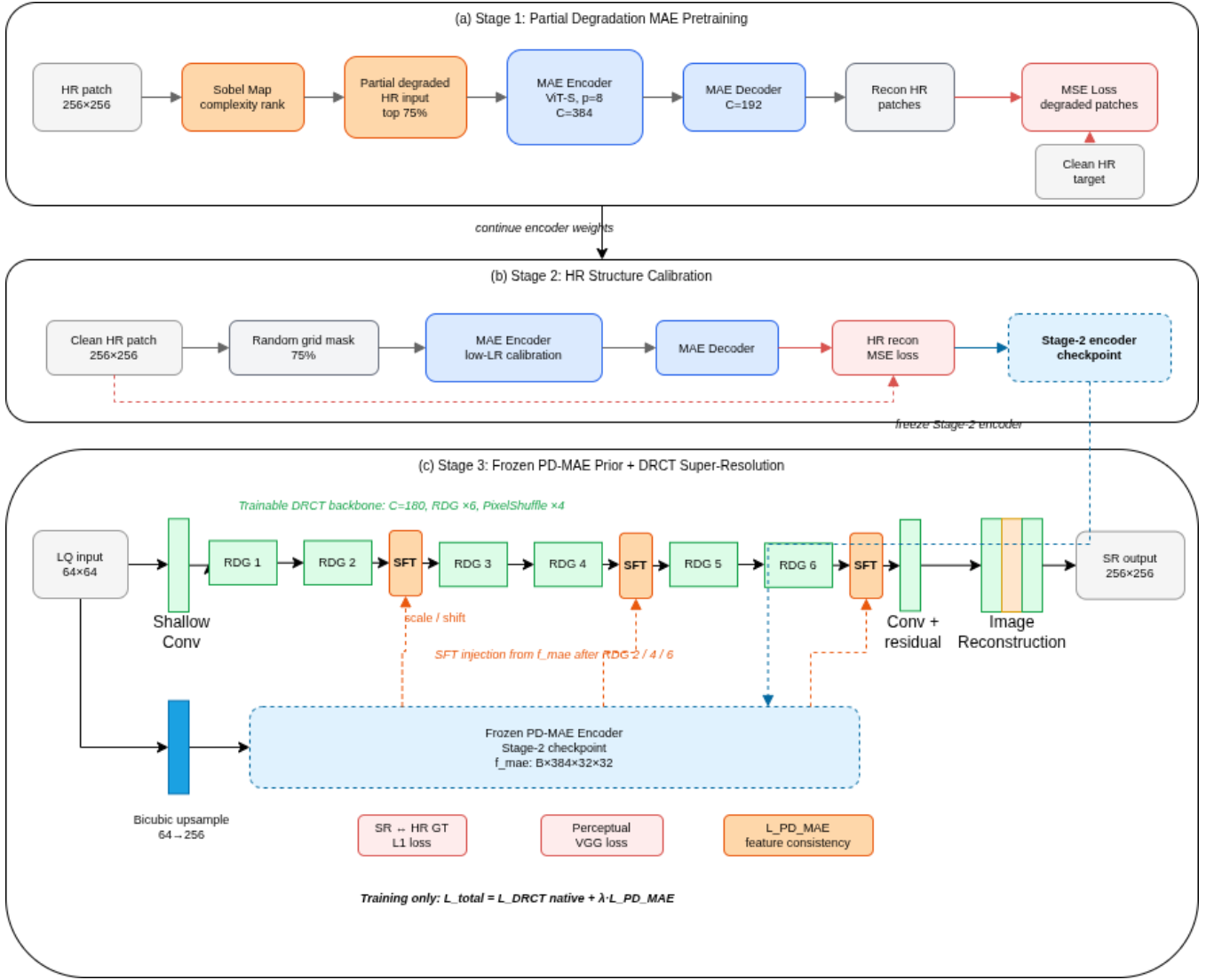
Fig. 1. Overall architecture of PD-MAE-DRCT. Stage 1 learns restoration-oriented priors through region-wise partial degradation; Stage 2 recalibrates the encoder on clean HR structure; Stage 3 freezes the PD-MAE encoder and injects its spatial prior into DRCT residual dense groups through SFT layers.
