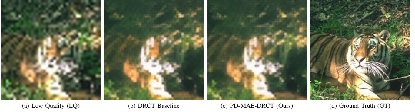
Fig. 5. Qualitative comparison on the BSDS100 (108070.png) dataset. Our method effectively reconstructs fine natural textures like tiger fur while maintaining high perceptual fidelity.
