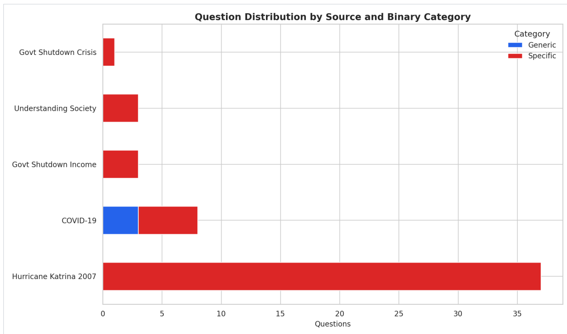
Figure 1: Binary Generic versus Specific distribution.
