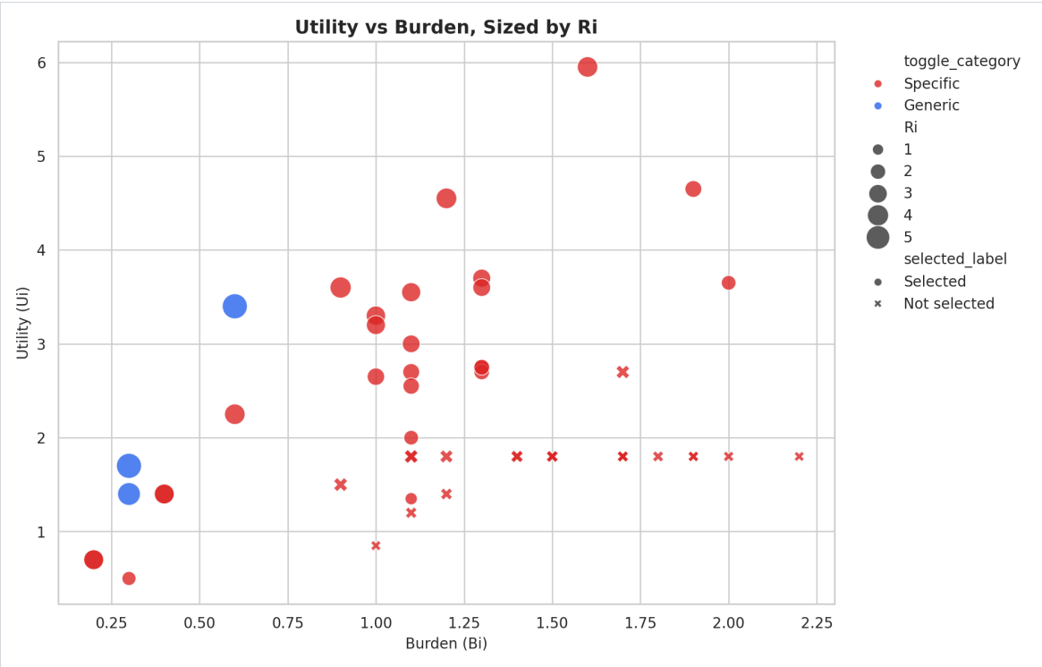
Figure 3: Utility-versus-burden relationship for the refreshed corpus.
