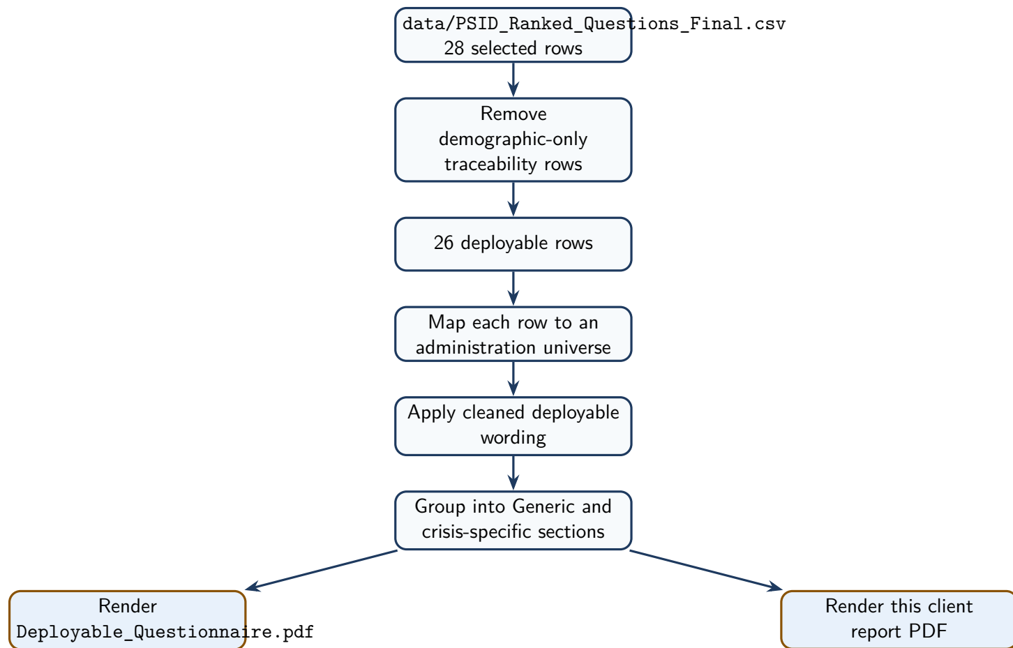
Figure 4: Operational path from the scored module to the deployable questionnaire package.
