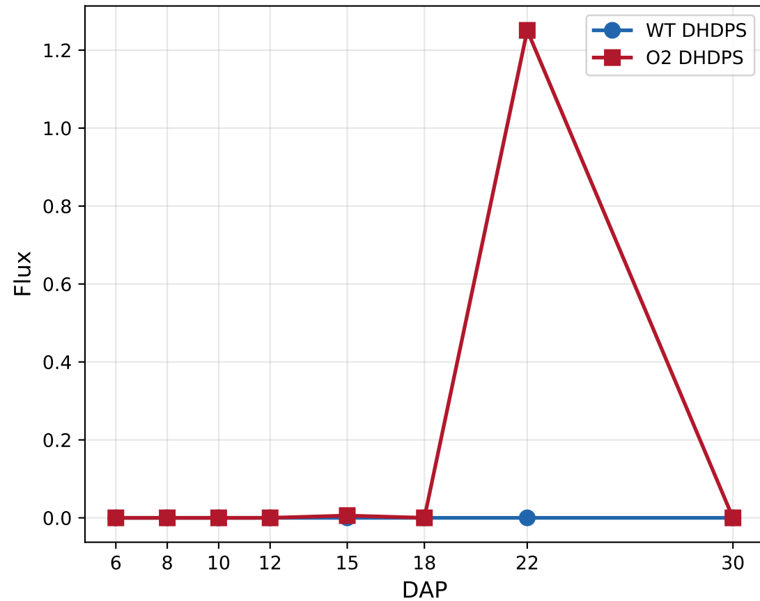
A. DHDPS (R02292) - Entry to Lysine Branch
