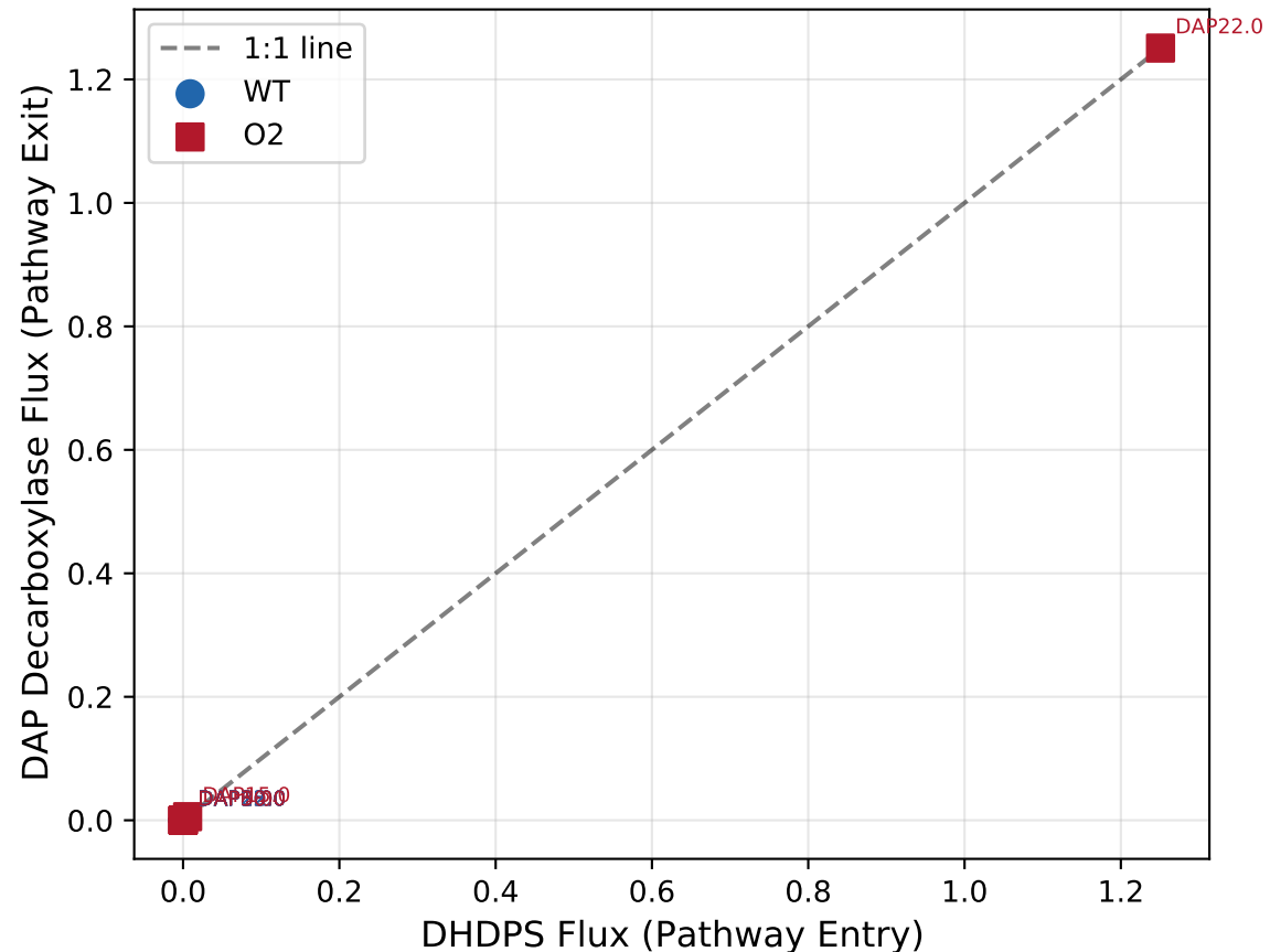
B. Pathway Entry vs Exit (Flux Coupling)
