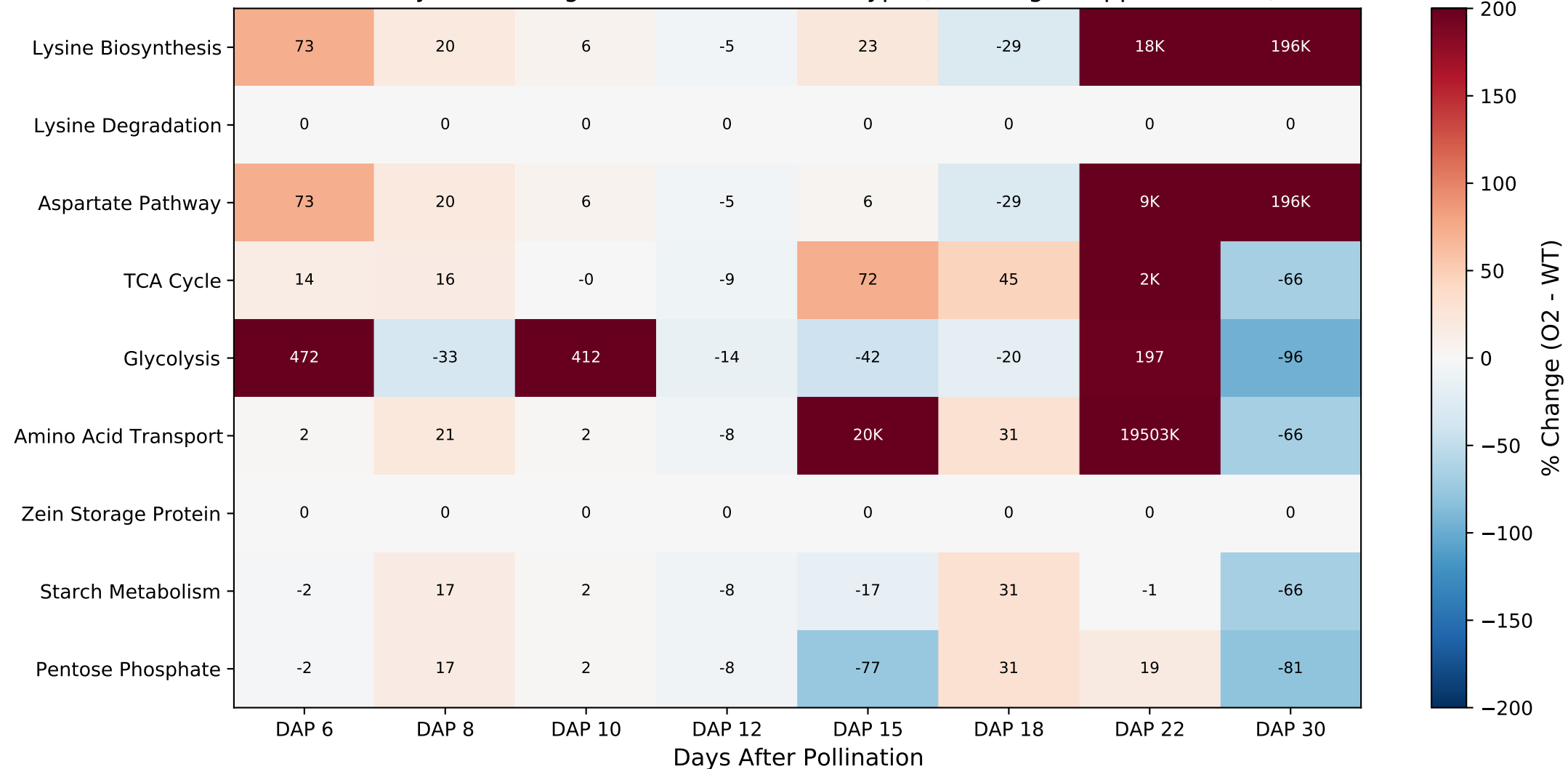
Pathway Flux Change: O2 Mutant vs Wild Type (% Change, clipped \pm 200\% )
