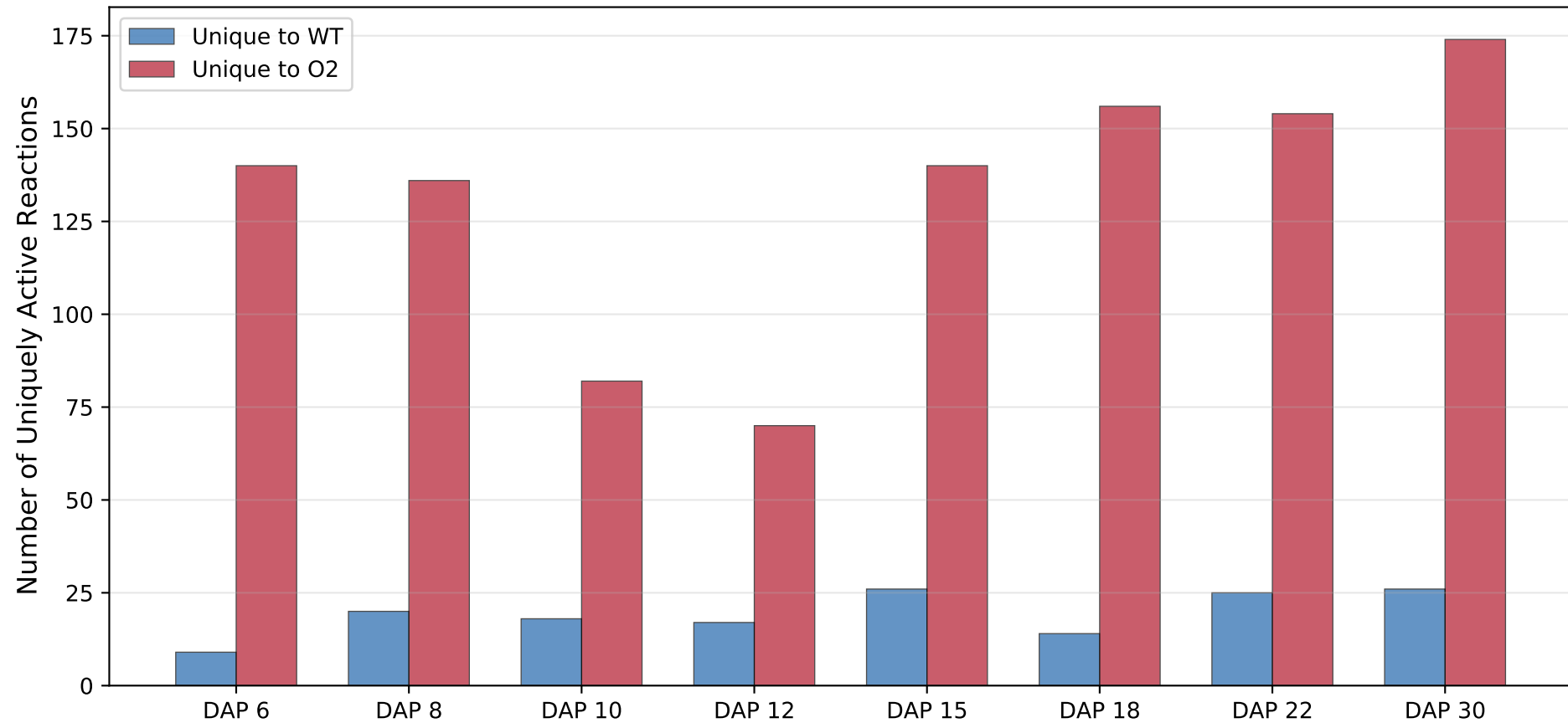
Reactions Active in Only One Genotype
