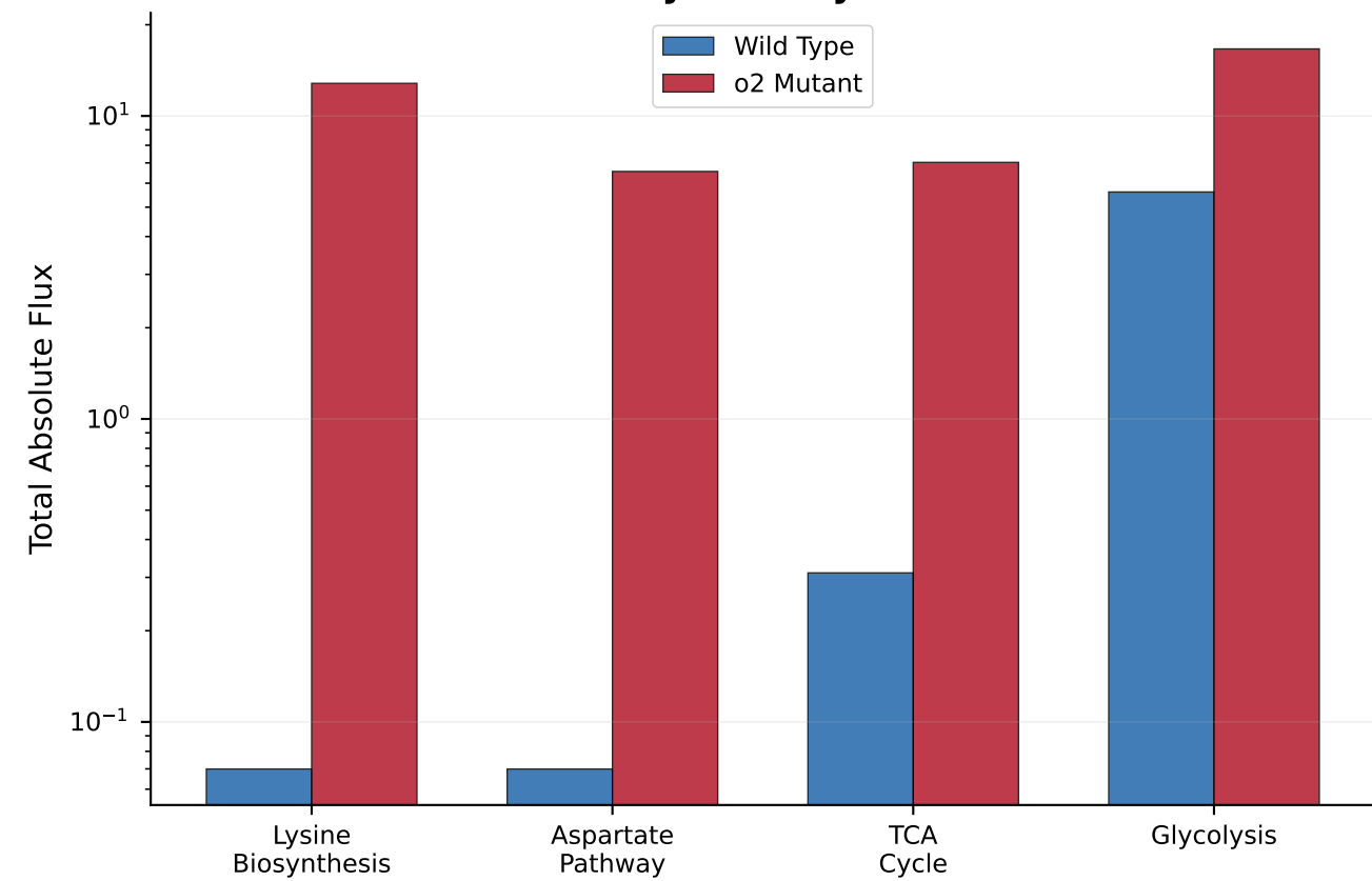
D. Pathway Activity at DAP 22
