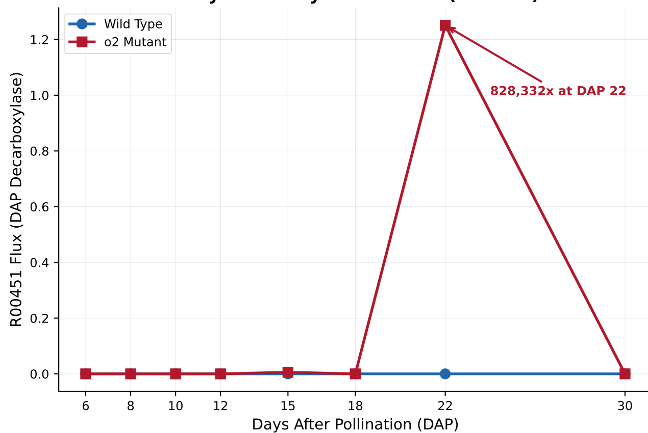
A. Lysine Biosynthesis Flux (R00451)
