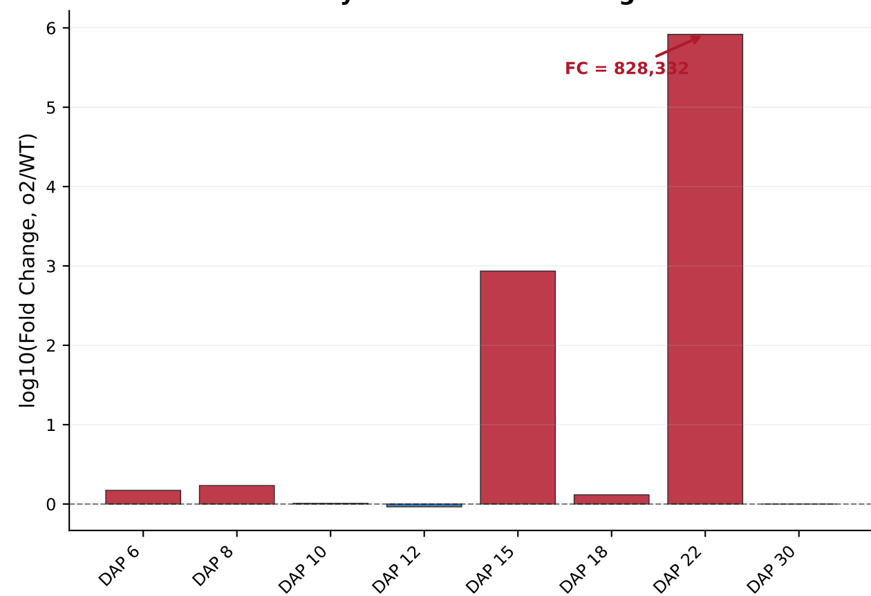
B. Lysine Flux Fold Change
