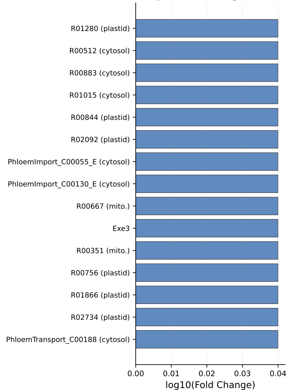
B. Overexpression Targets (2x Vmax)
