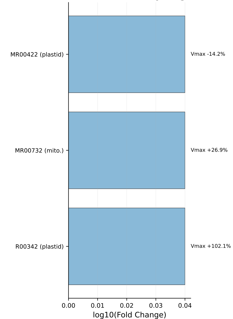
C. o2-Bound Mimicry Targets
