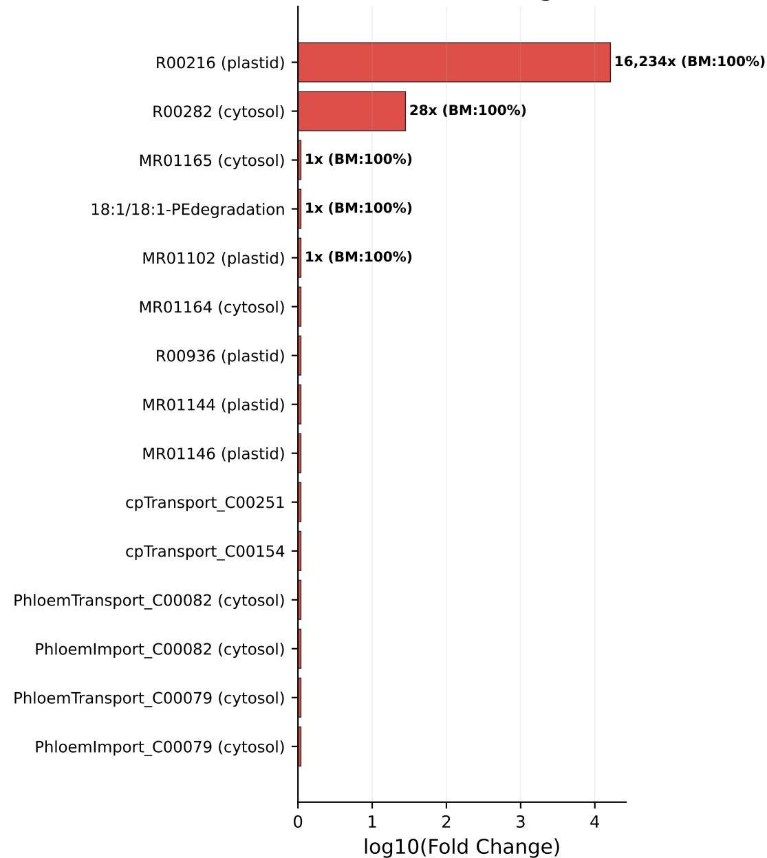
A. Knockout Targets
