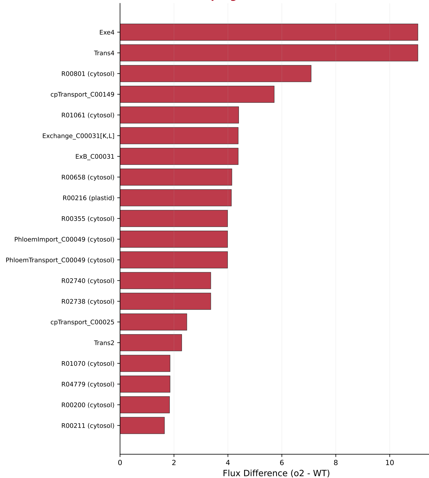
A. Upregulated in o2 at DAP 22
