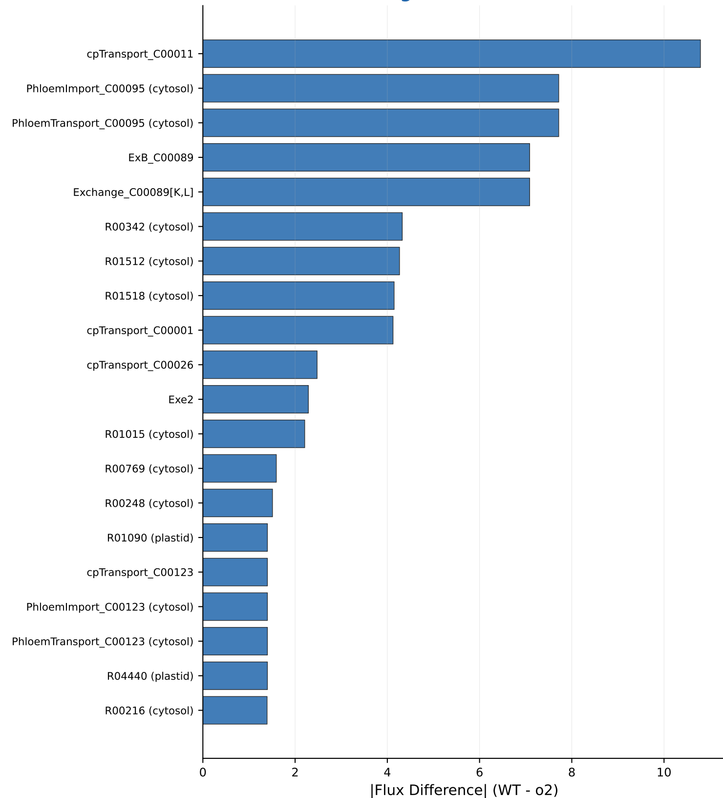
B. Downregulated in o2 at DAP 22
