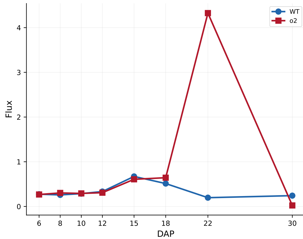
Phosphofructokinase GRMZM2G119300
