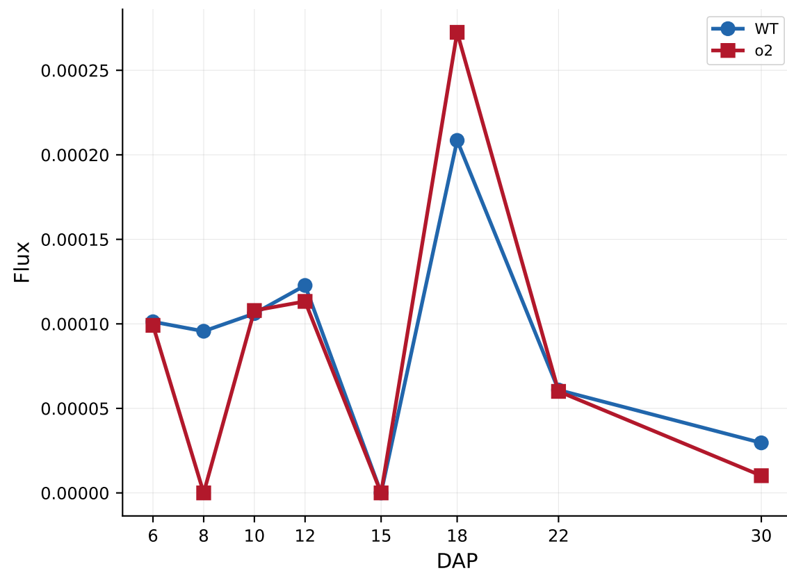
Phosphofructokinase GRMZM2G119300
