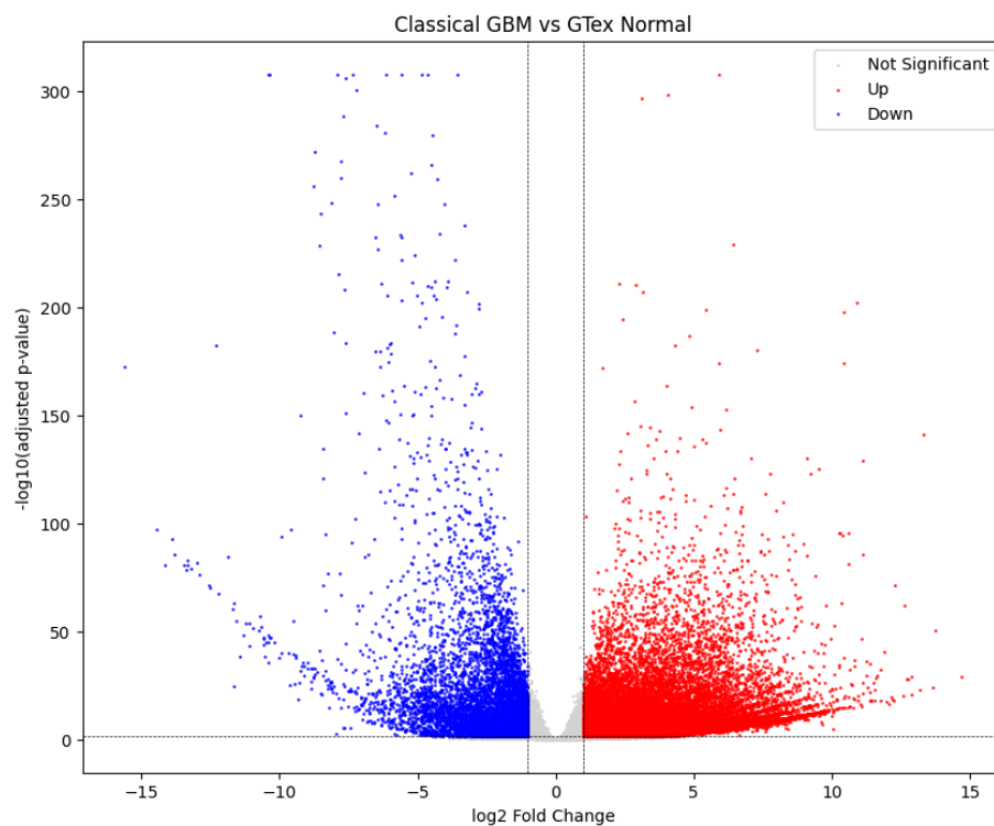
Figure 4.1. Classical GBM vs GTex Control Volcano Plot. There are 27.300 total significantly differentially expressed genes. More specifically, there are 20.300 significantly up-regulated genes (colored in red), and 7.000 significantly down-regulated genes (colored in blue).
