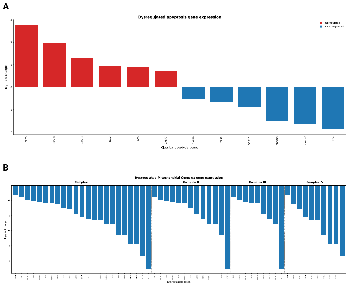
Figure 4.5. Log 2 FC bar graph of CYCS-interacting-protein encoding genes in (A) in apoptosis, and (B) respiratory complexes.
