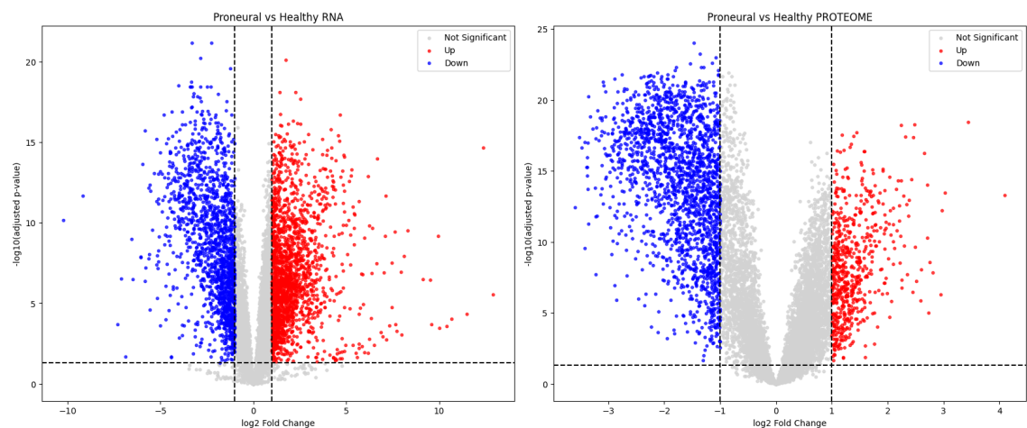
Figure 3.1. Example volcano plots. Left: Proneural Transcriptome. Right: Proneural Proteome.
