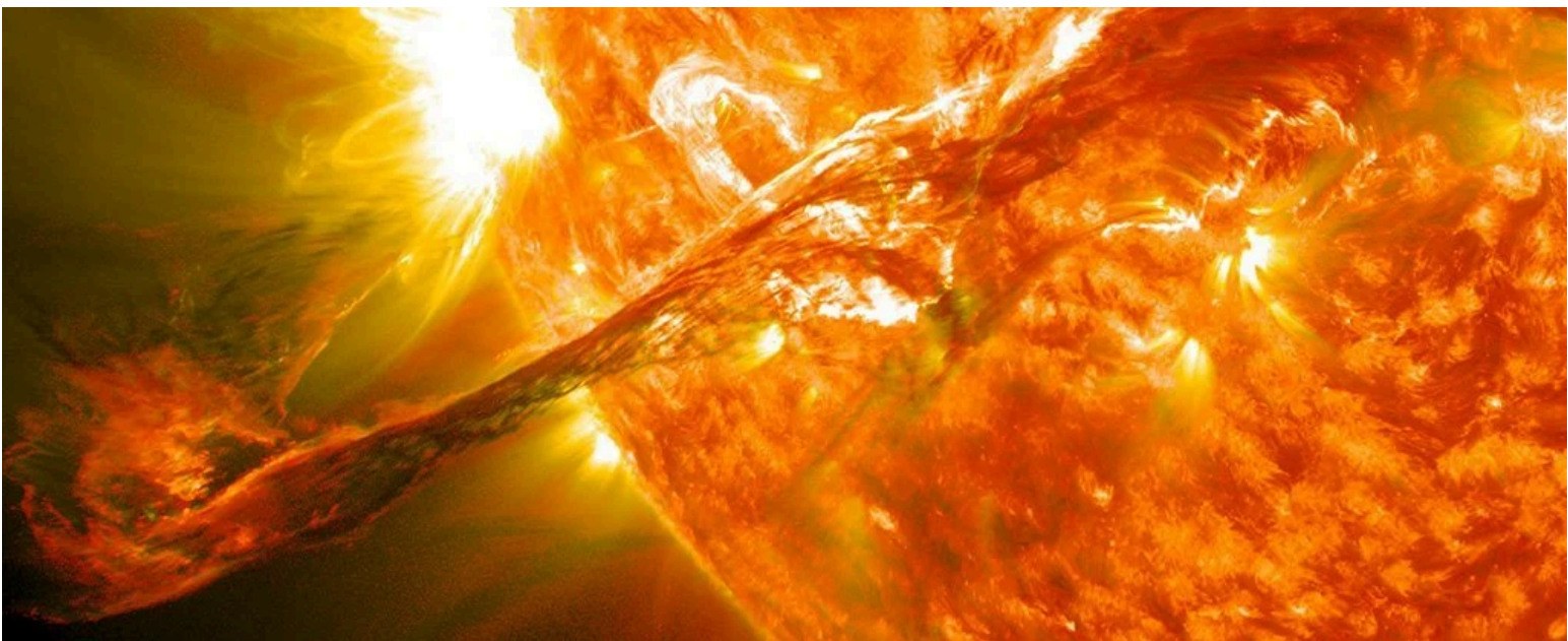
Figure 1: Coronal mass ejection observed by the Solar Dynamics Observatory at 304 Å on 2011 June 7.
