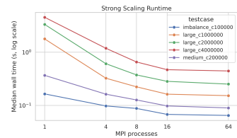
Figure 1: Strong-scaling run-time across process counts.
