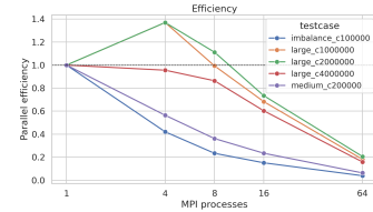
Figure 3: Parallel efficiency across process counts.
