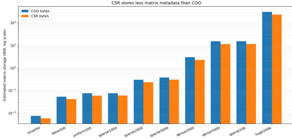
Figure 2: Estimated matrix storage (y-axis in log scale)
