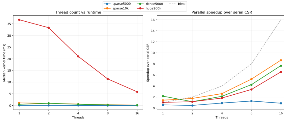
Figure 3: Thread scaling and speedup
