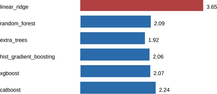
RT validation MAE (lower is better)
