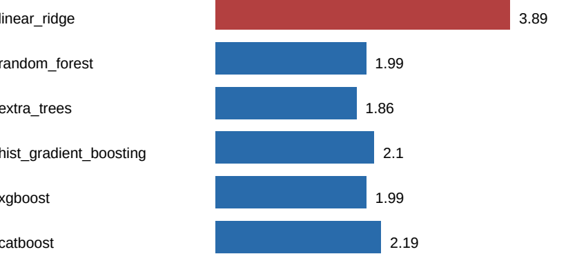
RT test MAE (lower is better)
