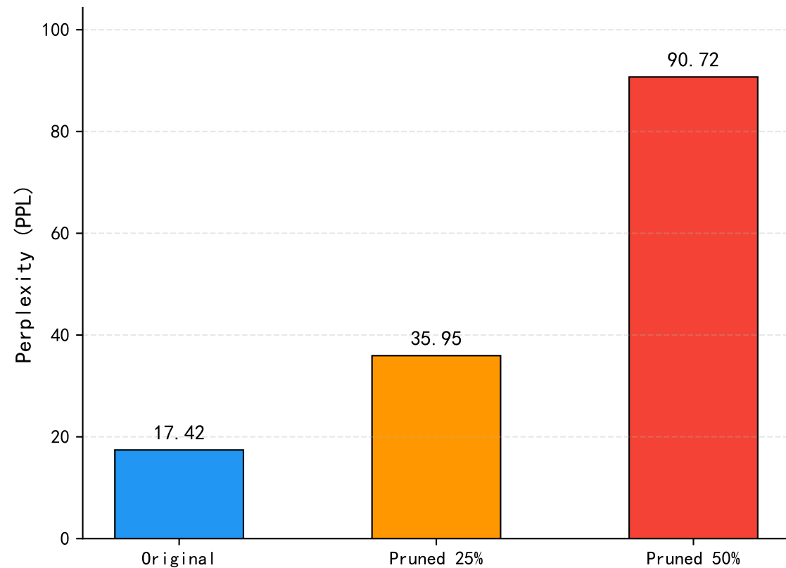
(a) PPL before and after pruning
