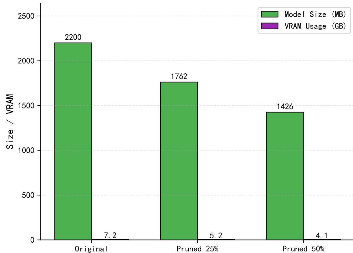
(b) Model size and VRAM usage
