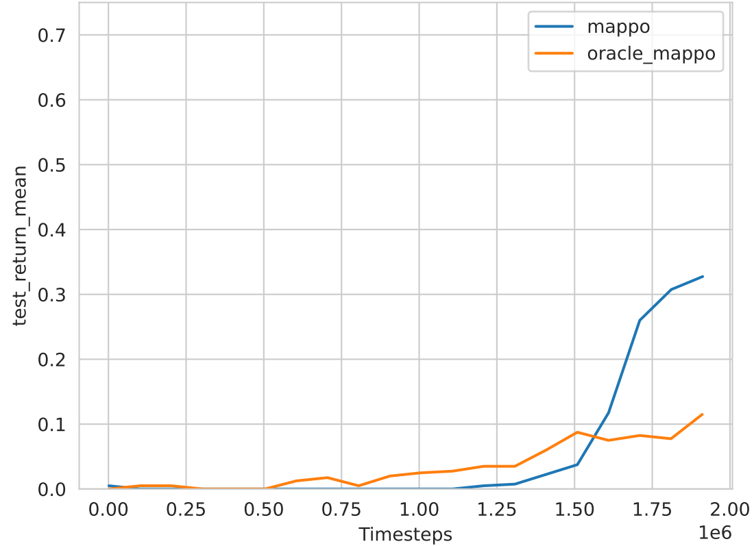
gymma_lbforaging:Foraging-2s-15x15-4p-4f-coop-v3 (common rewards; scalarisation sum)
