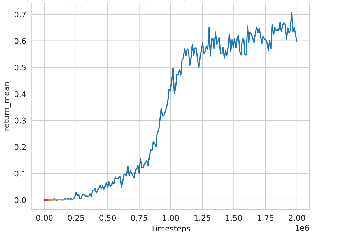
gymma_lbforaging-2s-10x10-3p-3f-coop-v3 (common rewards; scalarisation sum)
