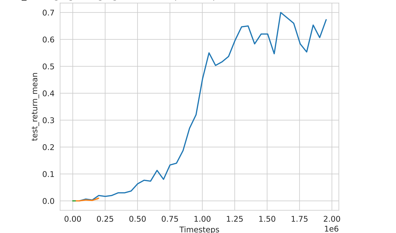
gymma_lbforaging-2s-10x10-3p-3f-coop-v3 (common rewards; scalarisation sum)
