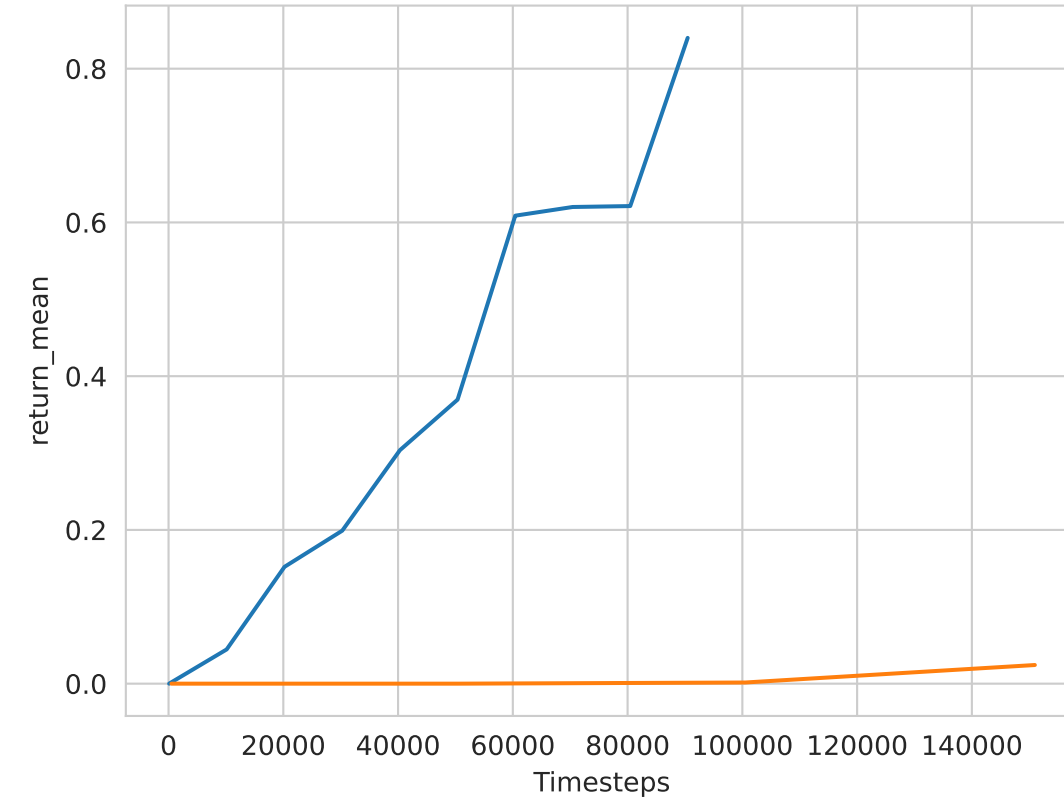
gymma_lbforaging:Foraging-2s-8x8-2p-2f-coop-v3 (common rewards; scalarisation sum)
