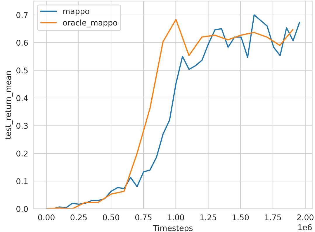
gymma_lbforaging:Foraging-2s-10x10-3p-3f-coop-v3 (common rewards; scalarisation sum)
