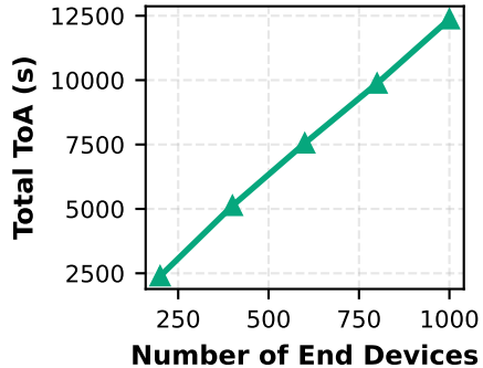
(c) Time on Air
