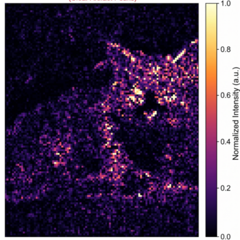
GAN HH Spectrum (Clear Artifact Peaks)
