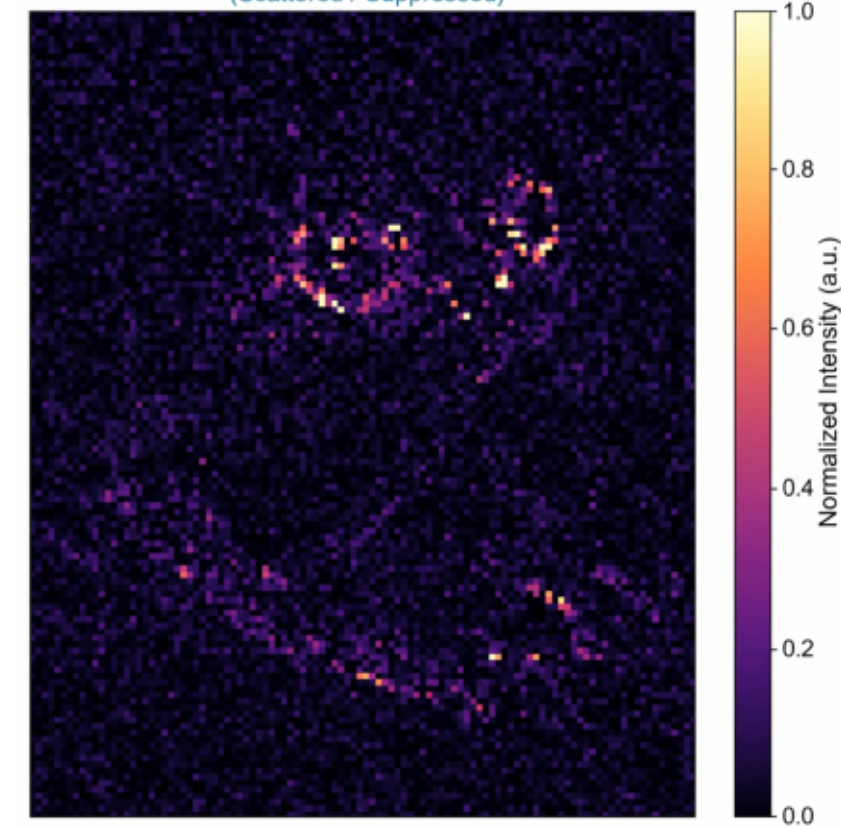
Diffusion HH Spectrum (Scattered / Suppressed)
