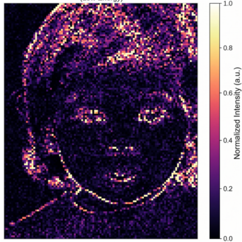
Real HH Spectrum (Low Energy)
