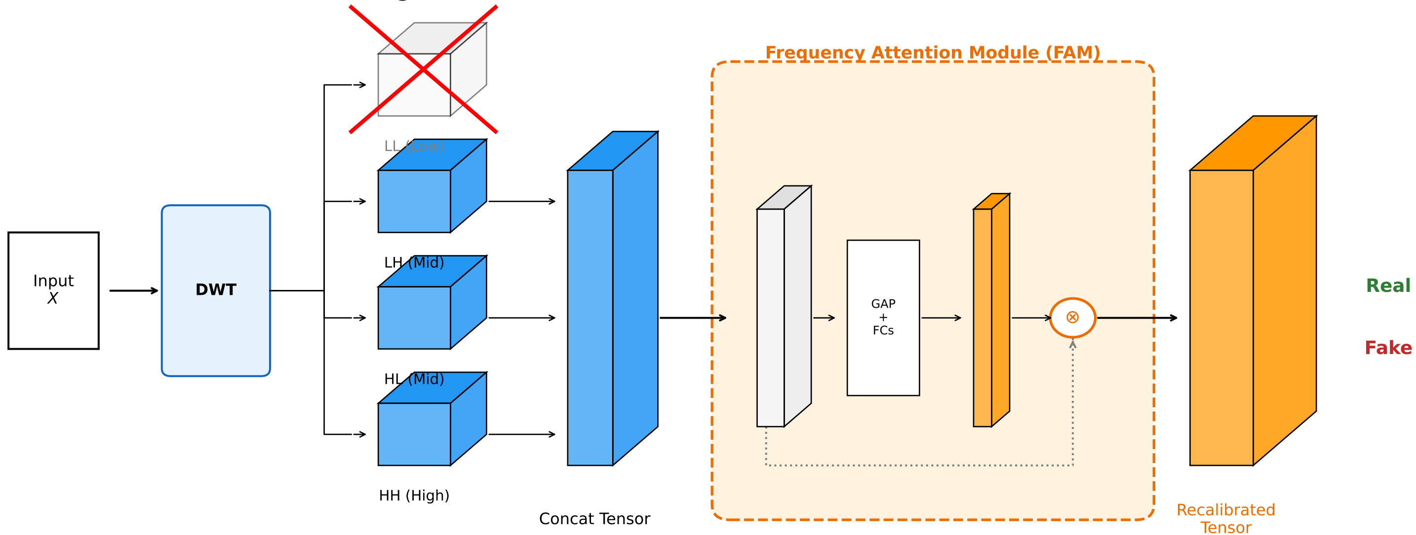
Figure 2: Overall Architecture of AMFF-Net (3D Tensors)
