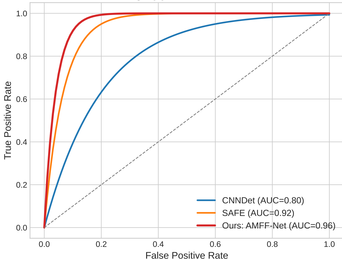
Fig 4(a): ROC on GANs
