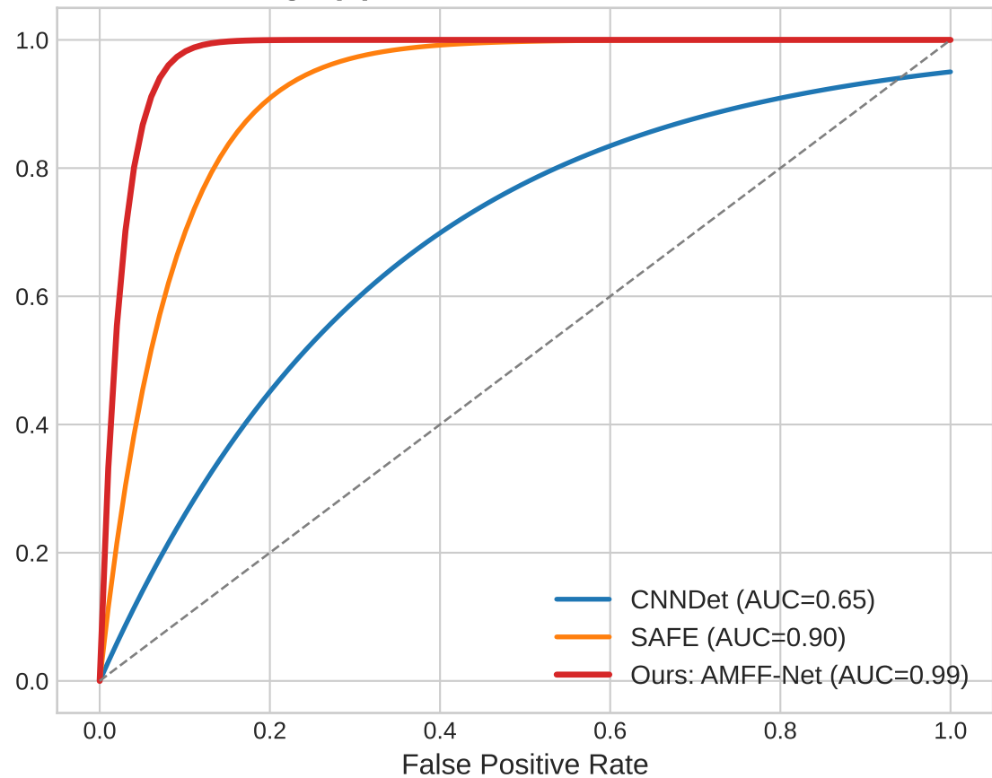
Fig 4(b): ROC on Diffusion Models
