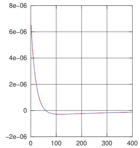
\pi^{F \circ W^*}
