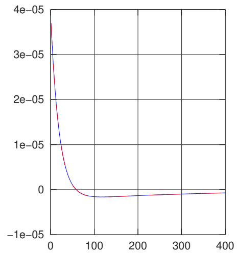
\pi^{H \circ W}
