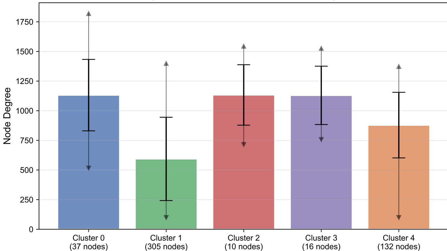
Degree Distribution by Risk Cluster (Bar = Mean \pm Std, Arrows = Min/Max)
