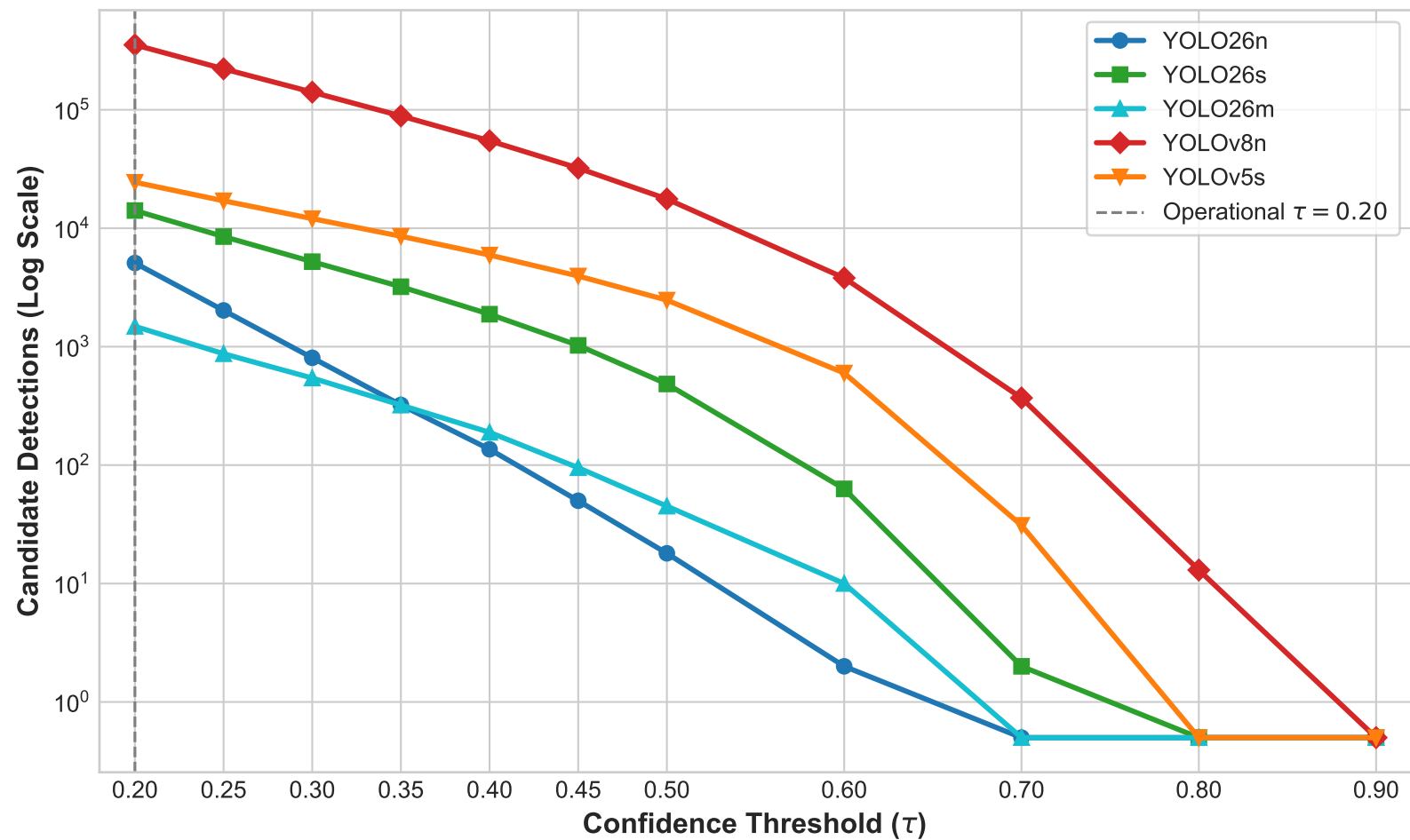
Target-Domain Candidate Detection Volume vs. Threshold
