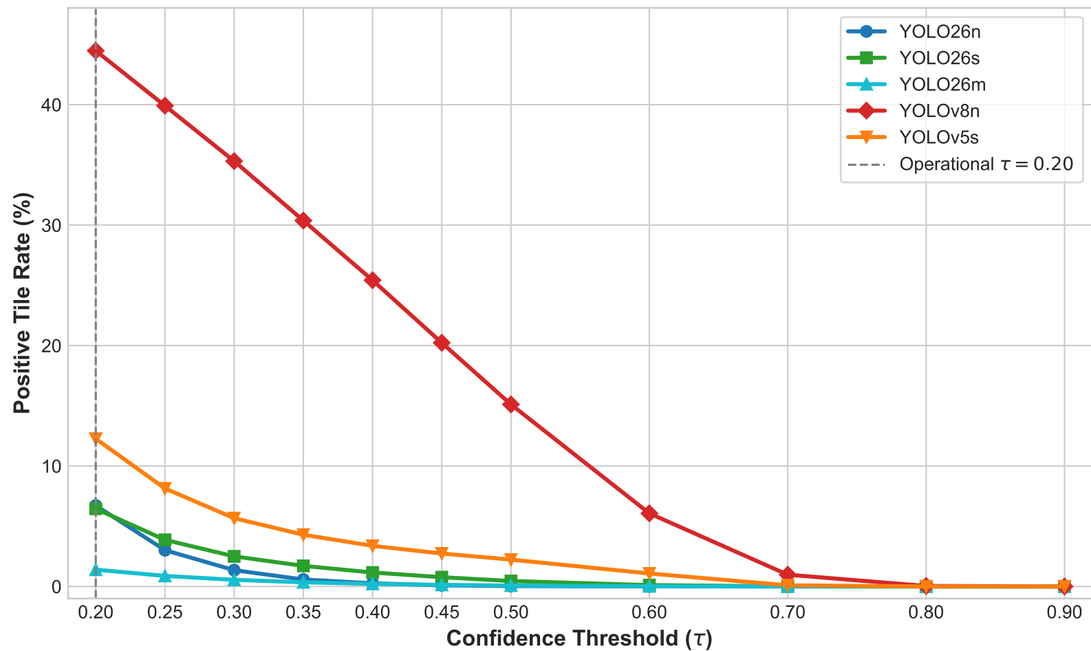
Target-Domain Positive Tile Rate Across Thresholds (N = 31,769 Tiles)
