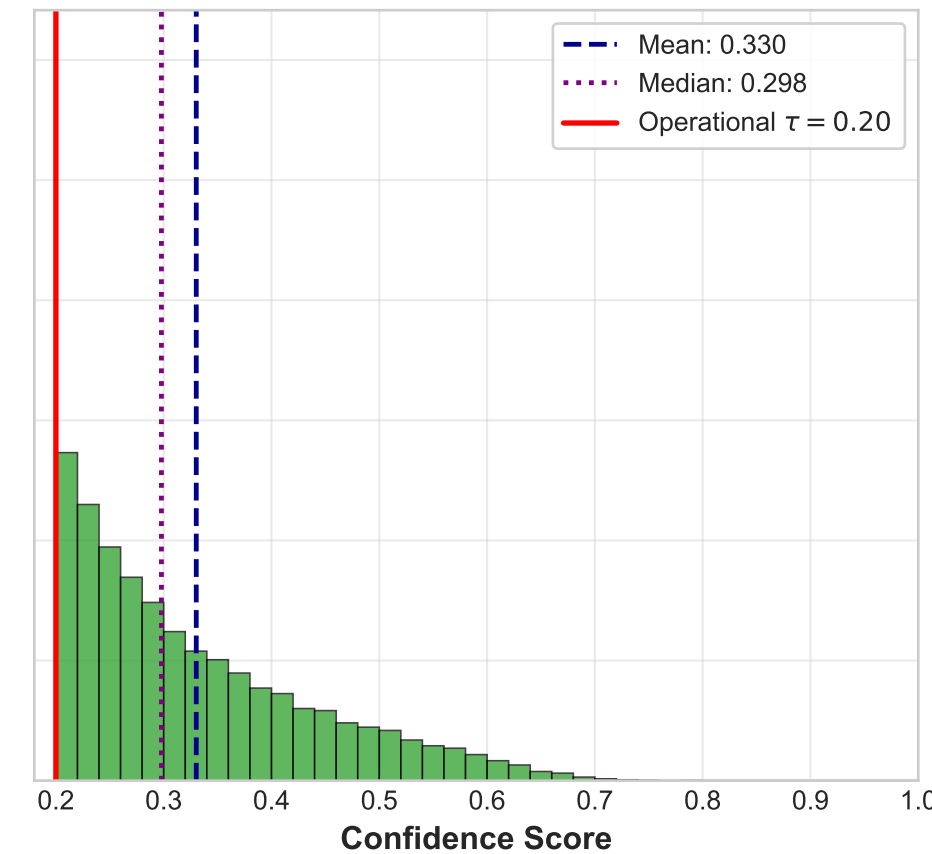
YOLOv5s (N = 24,452)
