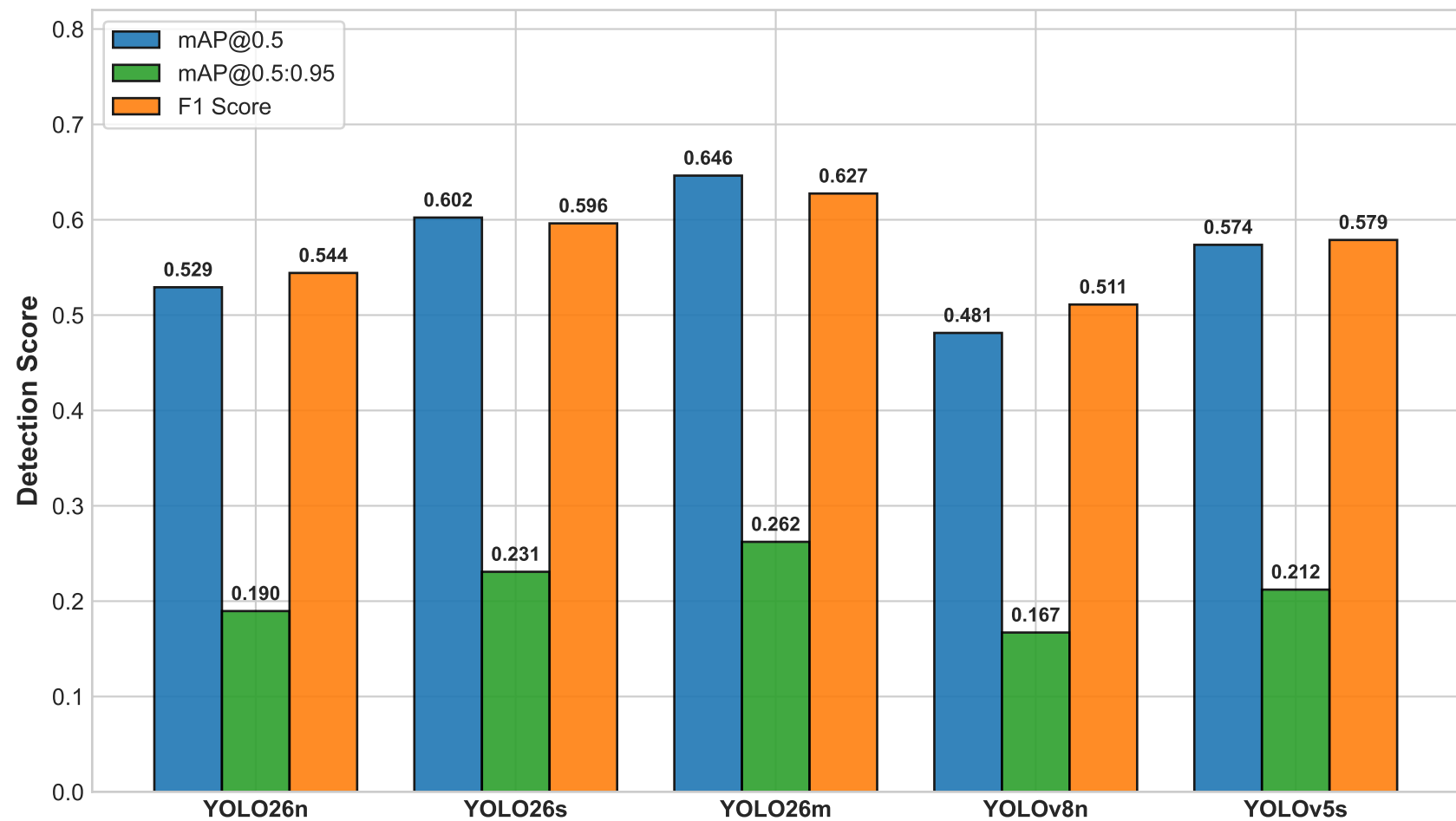
Source Test Metrics Across Model Scale & Architecture (HM Condition)
