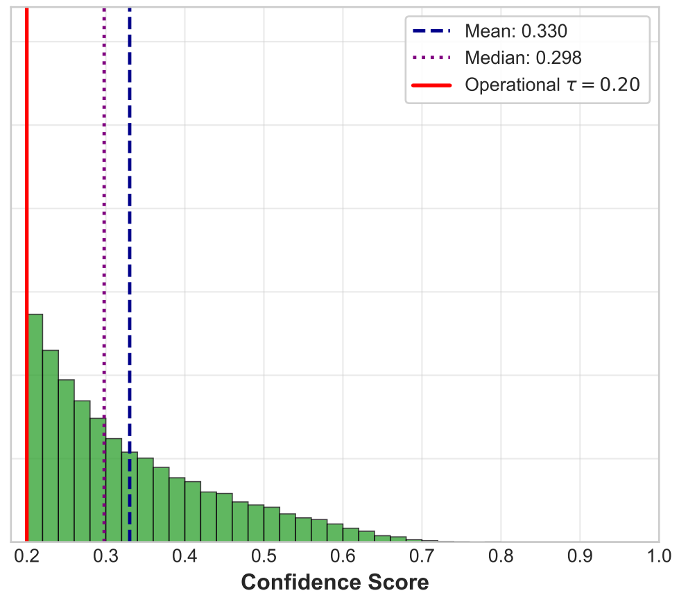
YOLOv5s (N = 24,452)
