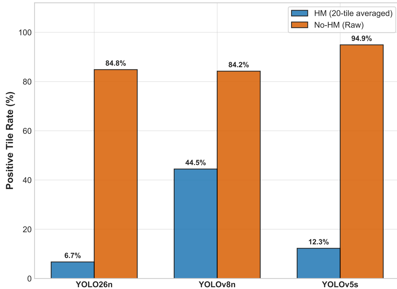
(a) Target-Domain Positive Tile Rate (N = 31,769 tiles)
