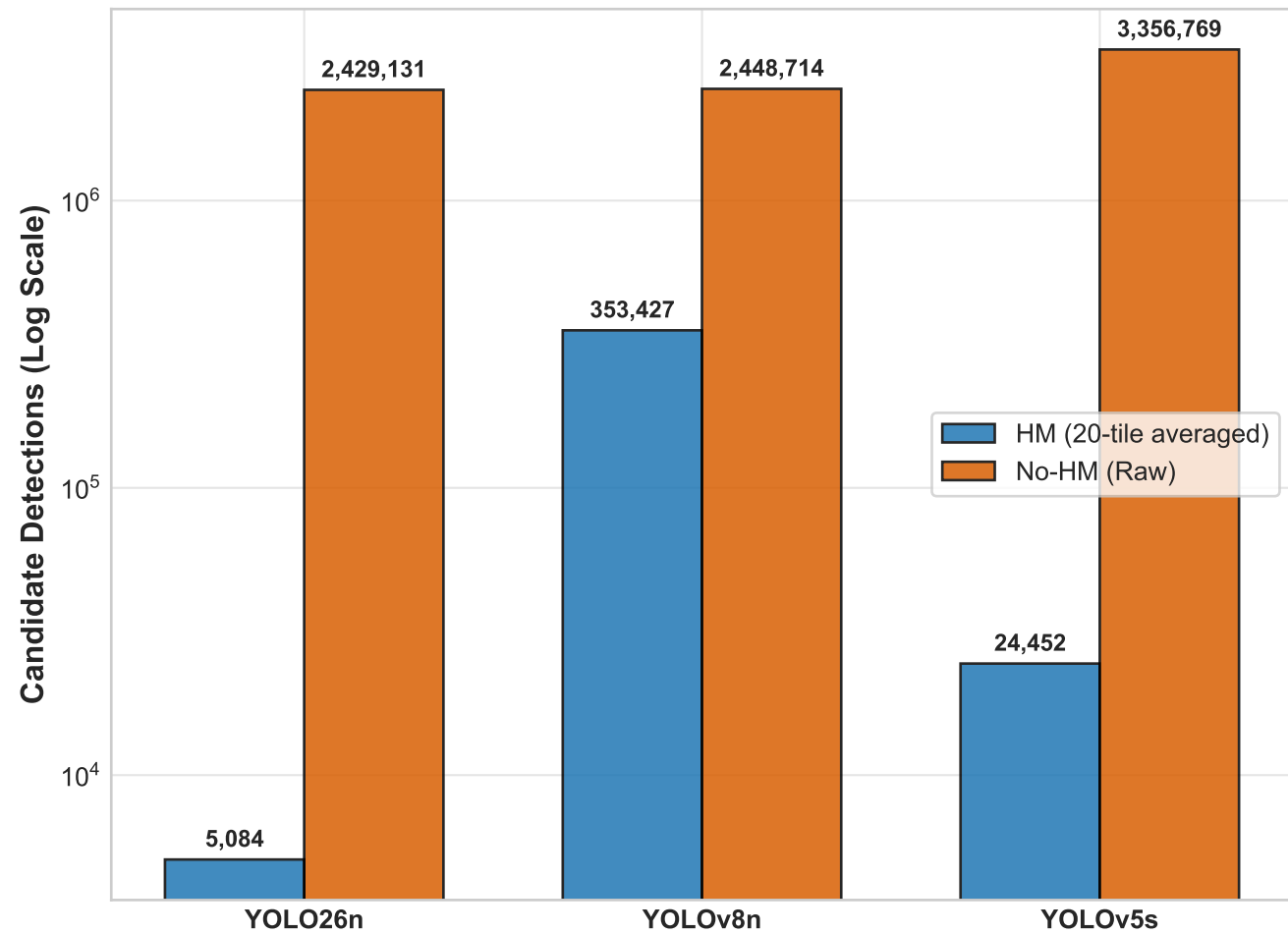
(b) Target-Domain Total Candidate Detections ( \tau = 0.20 )
