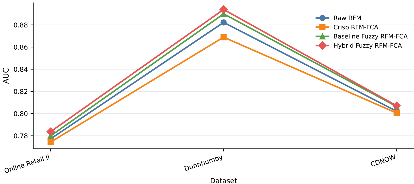
AUC comparison across RFM-FCA methods
