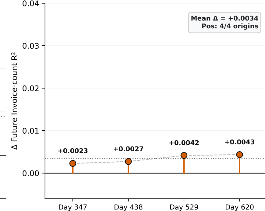
(f) Online Retail II · \Delta Future Invoice-count R^2
