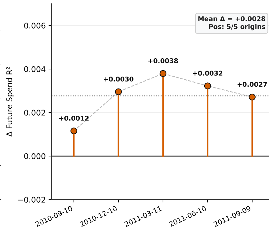
(e) Online Retail II · \Delta Future Spend R^2
