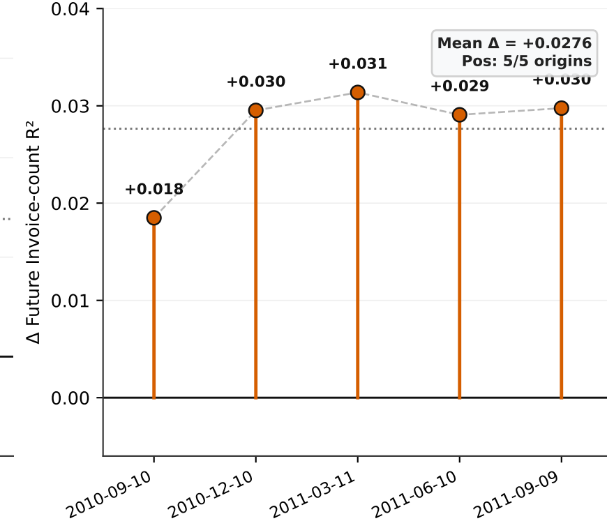
(f) Online Retail II · \Delta Future Invoice-count R^2
