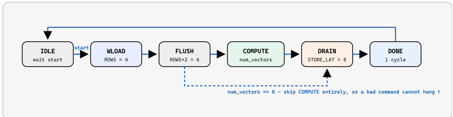
Figure 12.1 — the controller's six states. busy covers WLOAD...DRAIN. done is a single-cycle pulse fired in DONE, by which point busy is already low. start is sampled only in IDLE and is ignored while busy, so a stray pulse mid-job changes nothing.
