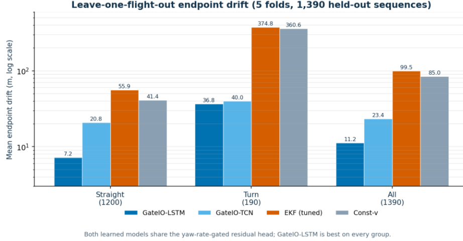
Figure 3. Leave-one-flight-out drift on a log scale. GateIO-LSTM stays below both classical baselines across groups, with the widest margin on turns; the convolutional backbone is worse.
