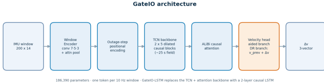
Figure 1. GateIO processes one token per 10 Hz window through a causal backbone and a two-branch velocity head.
