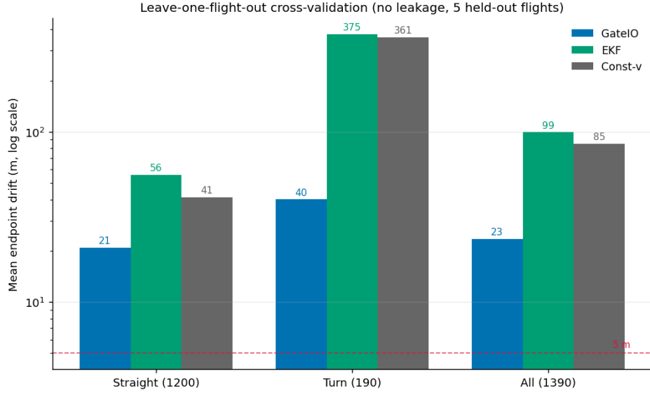
Figure 3. Leave-one-flight-out drift on a log scale. GateIO stays below both classical baselines across groups, with the widest margin on turns.
