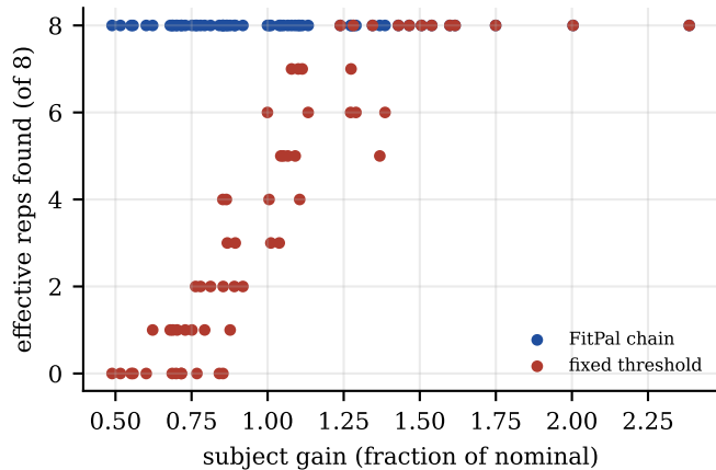
Sensitivity to electrode and subject gain
