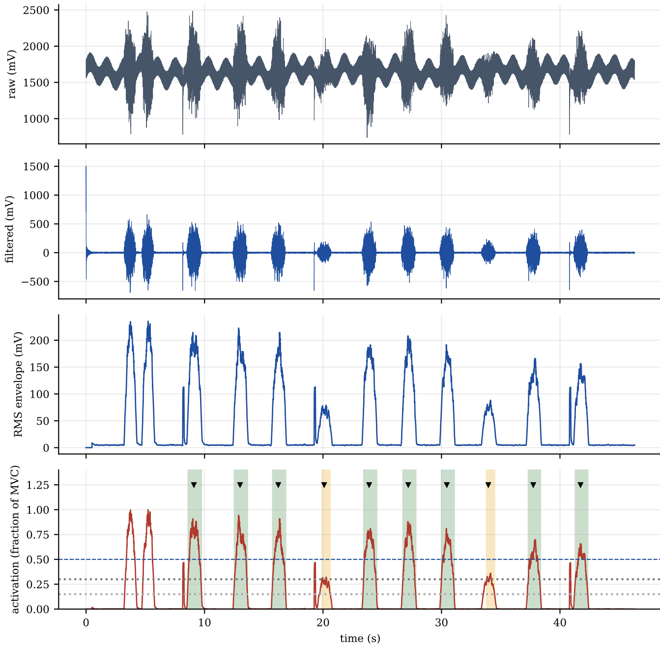
Simulated session: raw sensor voltage with hum, wander and motion spikes
