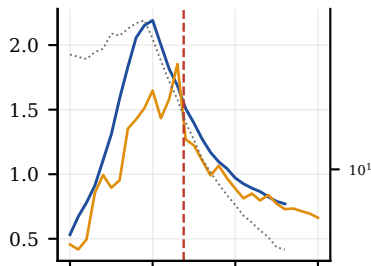
N = 64, f = 0.05
