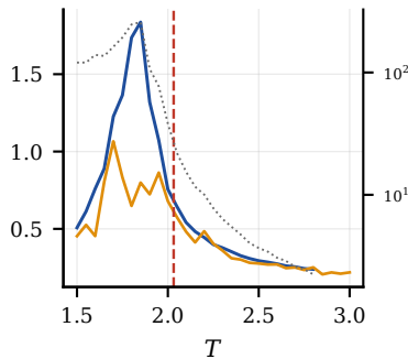
N = 64, f = 0.05
