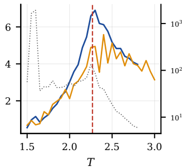
N = 64, f = 0.5
