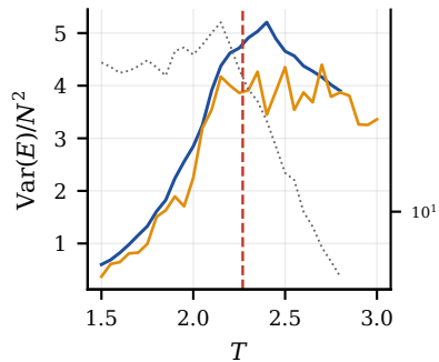
N = 32, f = 0.5
