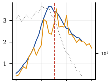
N = 64, f = 0.5
