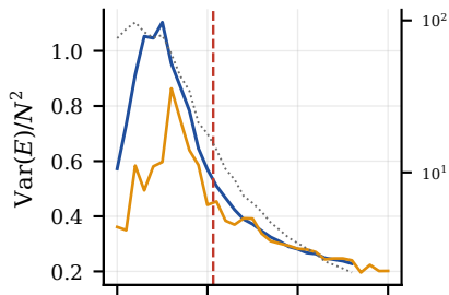
N = 32, f = 0.5
