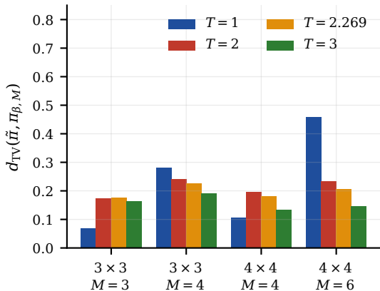
Uniform random-pair proposal (production)
