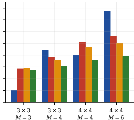
Nearest-neighbour proposal (classical Kawasaki)
