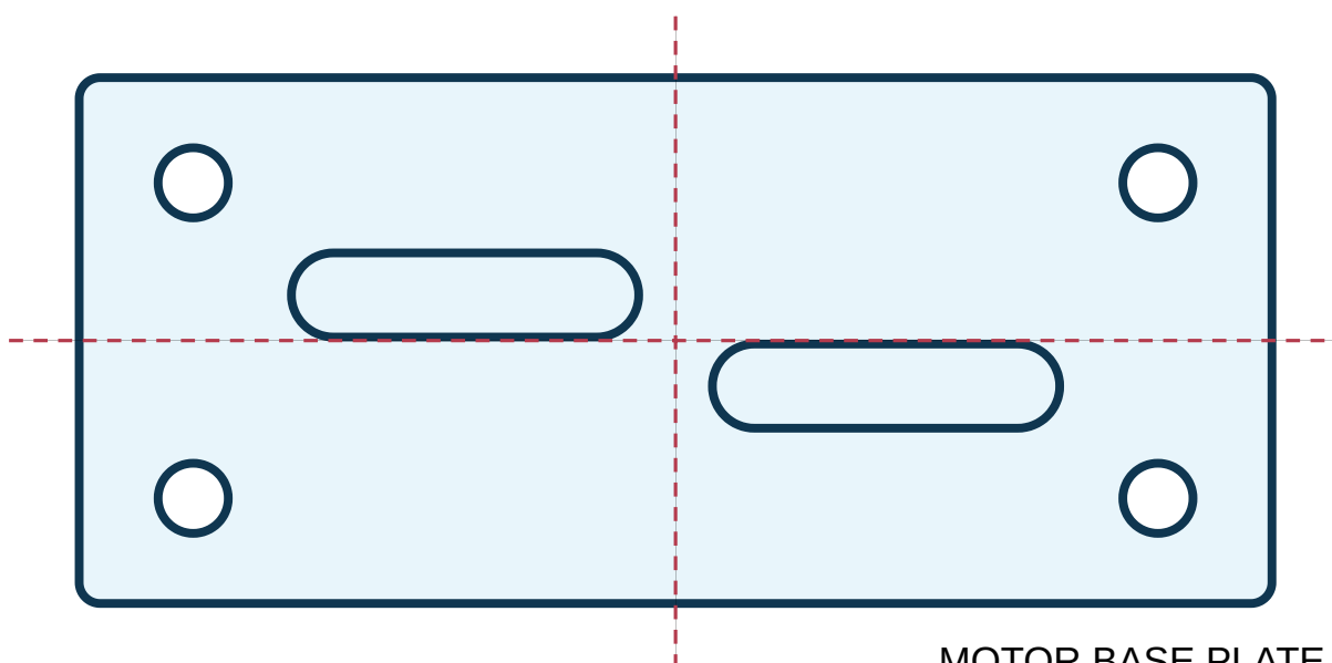
MOTOR BASE PLATE
