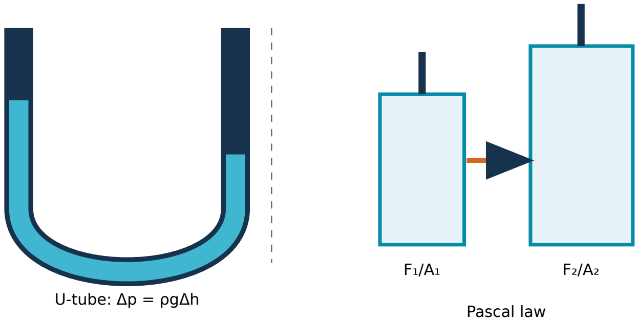
Figure 10. U-tube manometer. Reproduce the essential parts, labels and arrows in examination drawings.
