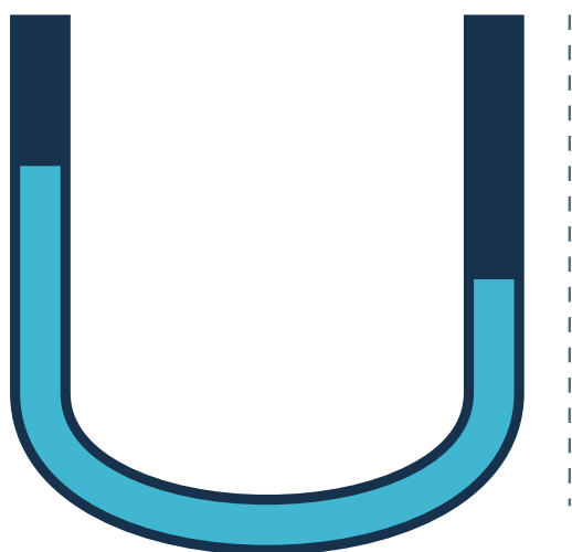
U-tube: \Delta p = \rho g \Delta h
